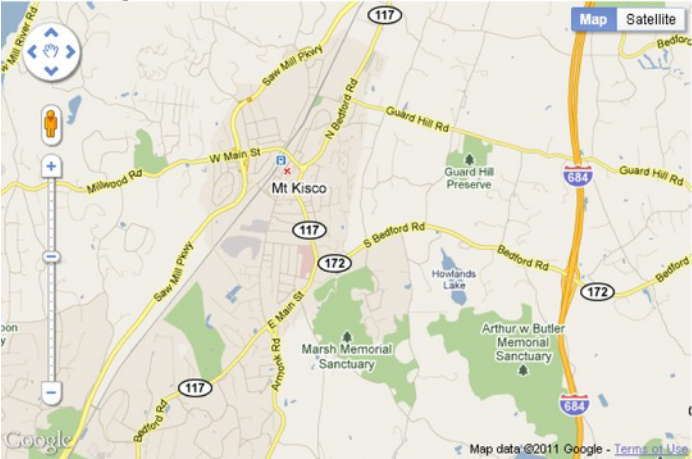
Figure 5-4. Image-and-audio combination
