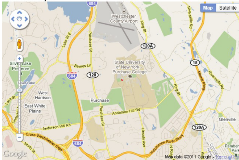
Figure 5-1. Opening screen
